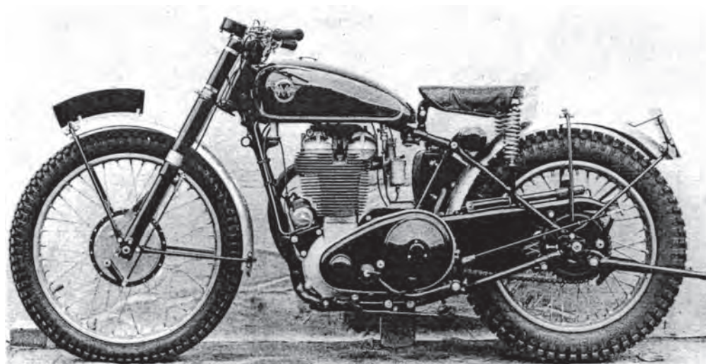
A maker's definitive photograph by courtesy of Motorcycle Sport for the 1953 500 cc Matchless. G80C shown here in trials guise with light-alloy motor, pre-Monobloc carburettor, rigid frame, Burman box and the AJS-style of forward mounted magneto introduced from September 1951. The Lucas instrument here is of course the Wader type. It has the new-type front brake brought in September 1952, the fullwidth front hub not arriving until 12 months later
