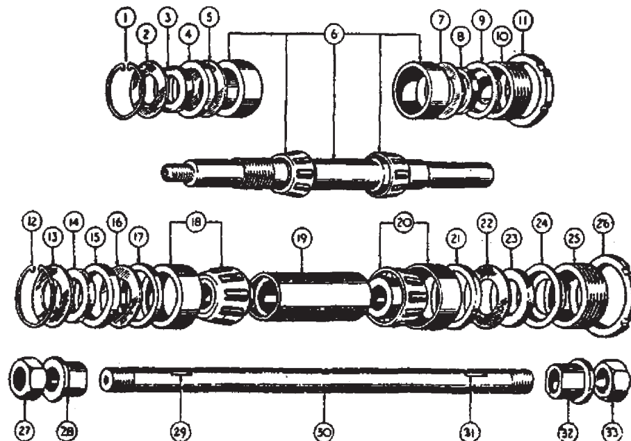
Post-war layout of wheel bearings showing (top) the front-wheel assembly and (bottom) rear hub components for spring-frame models
