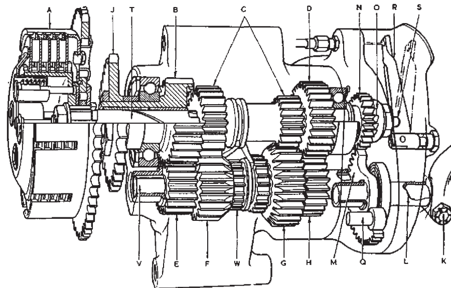
FIG 17 The CP-type Burman gearbox-clutch assembly
