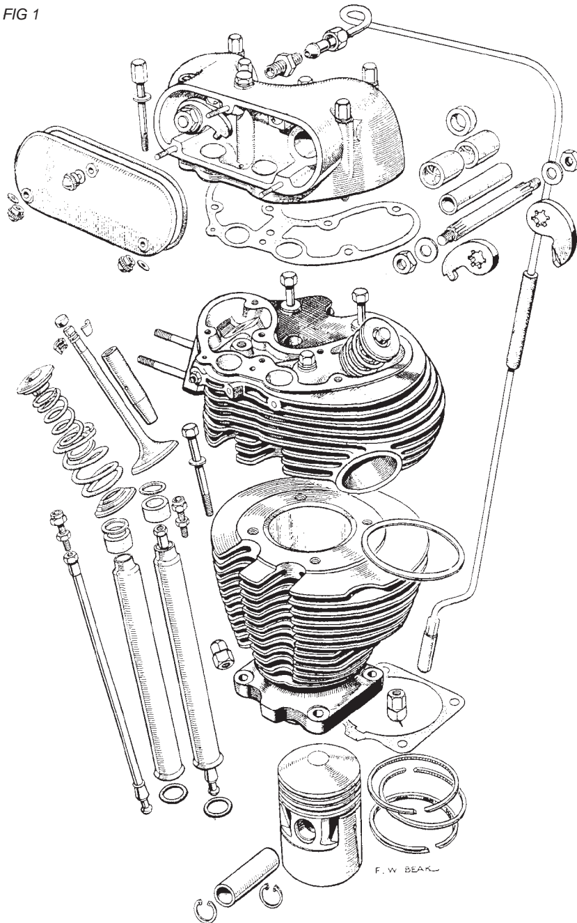
Top-half components of the Matchless WD-G3L circa 1941
